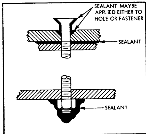
FIGURE 3.24.—Fastener sealing.
